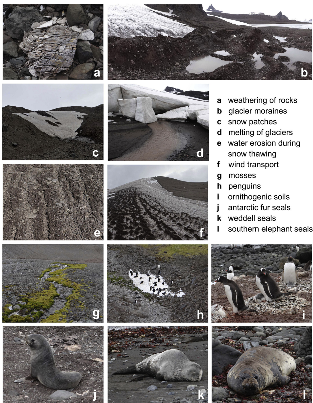
Fig. 6. Factors and processes influencing water chemistry characteristics.
