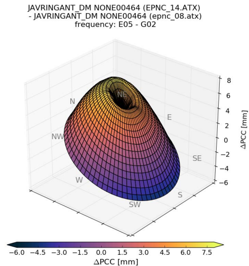
Fig. 9. Difference of antenna Phase Center Correction (PCC) between Galileo E5 and GPS L2 frequencies. Example for JAVRINGANT_DM NONE00464 antenna which is mounted at BRUX station.
