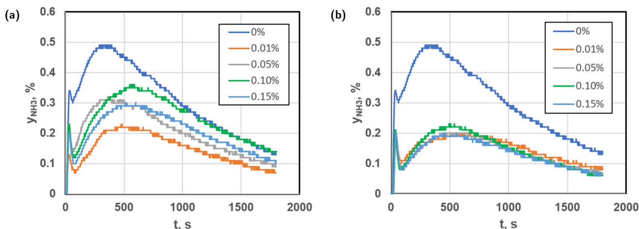
Figure 5. The volume fraction of ammonia in the outlet gas stream for selected experiments with: a) SiO 2 microparticles; b) colloidal SiO 2 particles.
