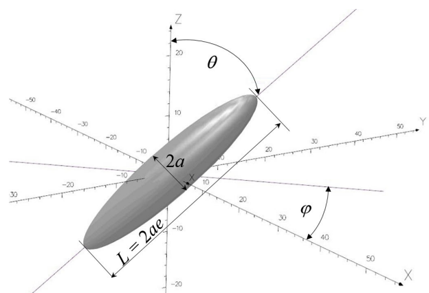
FIGURE 4. Virtual ferromagnetic object – longitudinal ellipsoidal shell.
