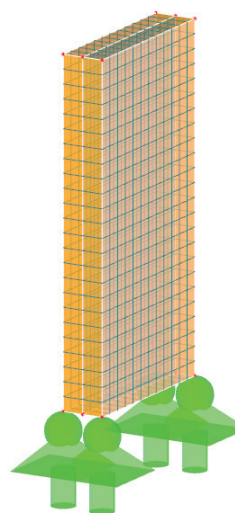
Fig. 2 Composite element with visible 3 layers of shell elements representing OSB sheathing and thermal insulation
