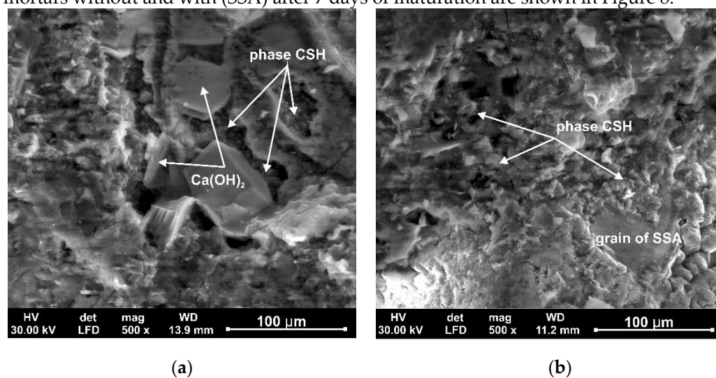
Figure 8. SEM microscopic image structures (500×): (a) OPC 42.5 R; (b) with sewage sludge ash after 7 days, magnification 500×.
