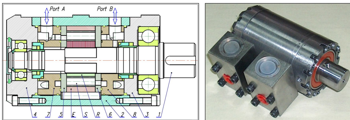
Figure 1. Tested motor (satellite motor) 22,37,38,46–48 . E—external gear (curvature), S—satellite, R—rotor, 1—shaft, 2,3 and 4—housing, 5 and 6—commutation plates (compensation plates), 7 and 8—inflow/outflow manifolds.
