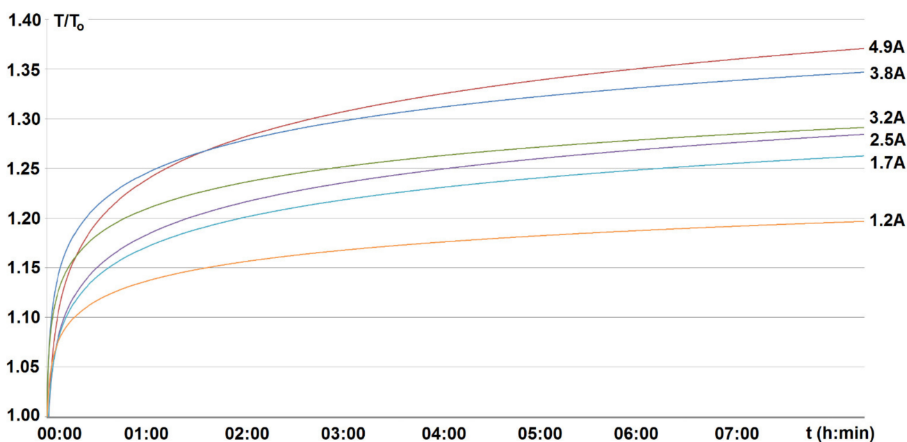
Figure 9. Increase in cell temperature T ( T_1 sensor) during discharge (to the minimum voltage value U_{\min} equal to 2.5 V) for various load currents under free room conditions. ( T_0 = 22 °C).
