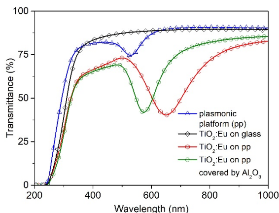
Figure 4. Transmittance spectra for TiO 2 :Eu thin film deposited on a Corning glass substrate and TiO 2 :Eu film deposited on plasmonic platform in both configurations, without and with additional dielectric layer. Additionally spectrum for plasmonic platform is presented.
