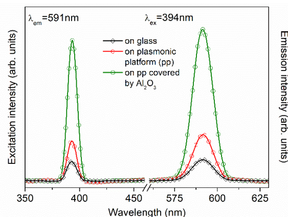
Figure 5. Excitation and emission spectra for TiO 2 :Eu thin film deposited on a Corning glass substrate and TiO 2 :Eu film deposited on plasmonic platform in both configurations, without and with additional dielectric layer.
