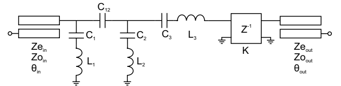
Fig. 2: Structure of the filter based on the coupling matrix. Elements values: Z_{e_{in}} = 76.68 \Omega , Z_{o_{in}} = 130.42 \Omega , \theta_{in} = 85.69^\circ at f_0 , L_1 = 2.04 nH, L_2 = 5.05 nH, L_3 = 5.29 nH, C_1 = 5.44 pF, C_{12} = 5.19 pF, C_2 = 1.6 nF, C_3 = 1.12 pF, K = 13.46 \Omega , Z_{e_{out}} = 77.92 \Omega , Z_{o_{out}} = 128.33 \Omega , and \theta_{out} = 88.7526^\circ at f_0 .
