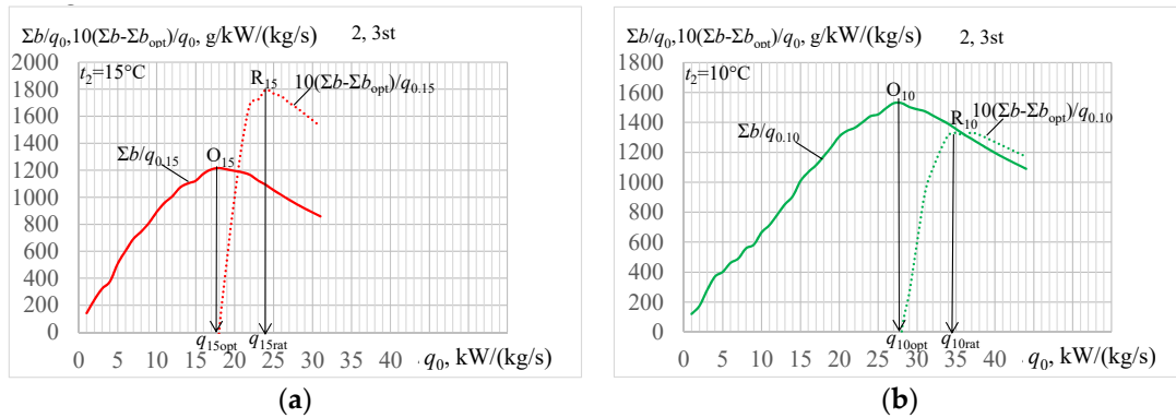
Figure 9. Relative increments of annual specific fuel reduction \Sigma b/q_0 and (\Sigma b - \Sigma b_{opt})/q_0 for t_{a2} = 15\text{ }^\circ\text{C} (a) and 10\text{ }^\circ\text{C} (b) against specific cooling capacity q_0 .
