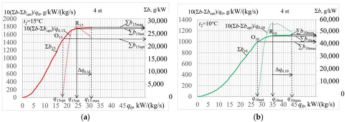
Figure 10. Annual specific fuel reduction \Sigma b and relative increment of annual specific fuel reduction (\Sigma b - \Sigma b_{opt})/q_0 for t_{a2} = 15\text{ }^\circ\text{C} (a) and 10\text{ }^\circ\text{C} (b): -(\Sigma b - \Sigma b_{opt})/q_0 .
