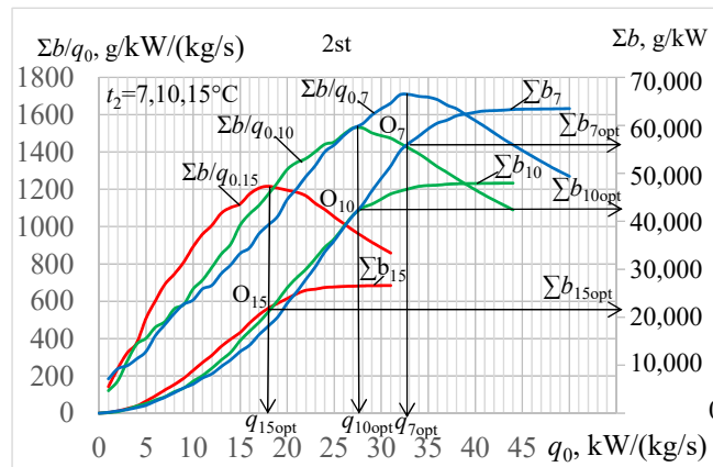
Figure 11. Relative increment of annual specific fuel reduction \Sigma b/q_0 and annual specific fuel reduction \Sigma b due to cooling air to t_{a2} = 7, 10 and 15\text{ }^\circ\text{C} against a cooling capacity needed q_0 (2 stage of methodology).
