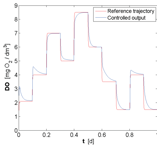
Fig. 13. Closed loop system performance before calibration.
