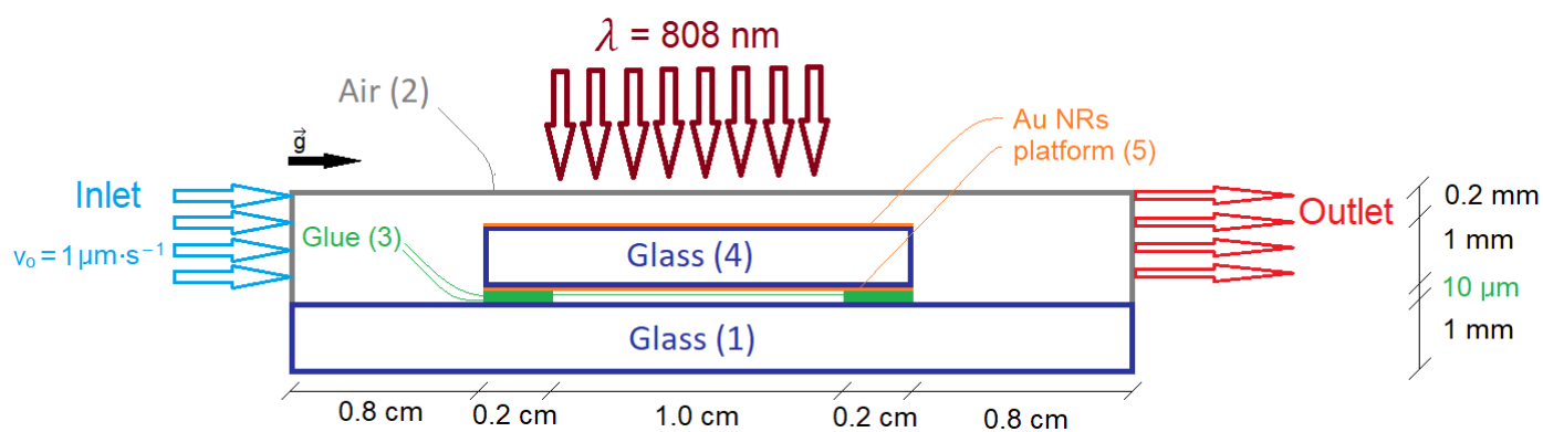
Figure 4. Scheme and dimensions of the gold nanorod platform from side view (scale has not been saved).
