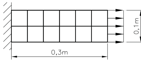
Fig. 4. Geometry and load imposing of a bar
