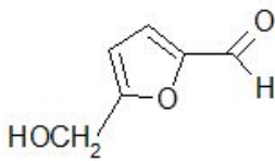
376 Fig. 9. Chemical structure of 5-hydroxymethyl-2-furaldehyde (HMF)
