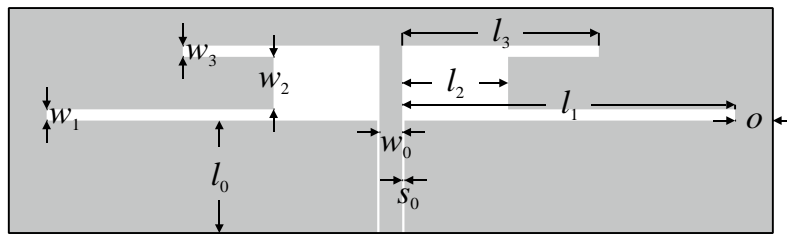
Fig. 10. Dual-band dipole antenna geometry [74].
