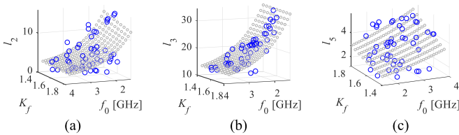
Fig. 17. Dual-band power divider of Fig. 16: inverse regression model for selected geometry parameters: (a) l_2 , (b) l_3 , and (c) l_5 . Inverse model surfaces and random observables are shown using gray and blue circles, respectively.
