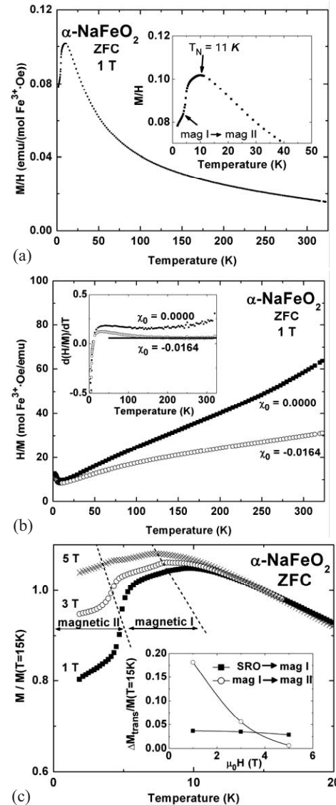
FIG. 8. (a) The magnetic transitions in \alpha -NaFeO 2 can be seen in the zero field cooled magnetic-susceptibility data at \mu_0 H = 1 T. The Néel point coincides with the appearance of the magnetic I phase in the neutron data. A change in slope in the susceptibility around 5 K is concomitant with the transition from the magnetic I to the magnetic II phase. (b) \alpha -NaFeO 2 does not follow the Curie-Weiss behavior up to 320 K, even with a \chi_0 term. (c) Magnetization curves normalized to the values at T = 15 K show the suppression of the magnetic I to magnetic II phase transition.
