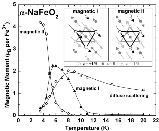
FIG. 7. Sodium ferrite displays two long-range-ordered magnetic phases as well as short-range magnetic correlations. The moment per Fe 3+ was extracted from fits of the diffuse scattering and Rietveld refinement at each temperature. The inset shows the ordering of the moments in the magnetic I and magnetic II phases as determined by neutron refinements.
