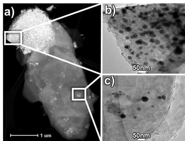
Figure 5. (a) HAADF image of a SiOC:C 0.2 /Sn-60% particle with separated ceramic and graphitic phases; TEM images of (b) ceramic phase and (c) graphitic phase.
