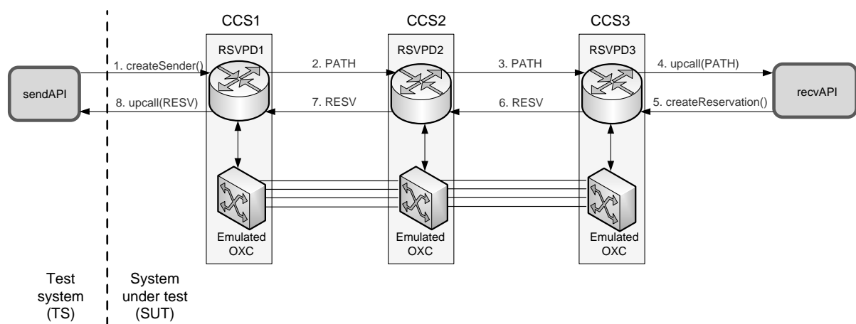
Fig. 3. ASON/GMPLS testbed architecture.
