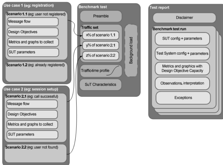
Fig. 1. ETSI performance measurements information model [6].
