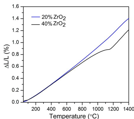
Figure 8. Shrinkage behavior of \text{Al}_2\text{O}_3 –(20,40 wt %) \text{ZrO}_2 nanocomposites.
