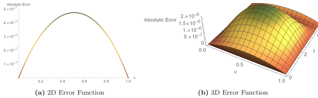
Fig. 7 2D and 3D error profiles when N = 32 , \Delta t = 0.01 , \gamma = 0.5 , t = 5 and v \in [0, 1] for Example 12.
