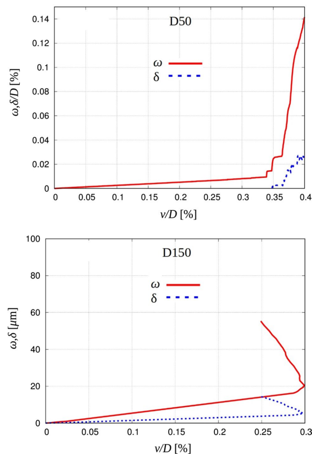
Fig. 13 DEM results: evolution of crack displacement versus normalized vertical displacement v/D in macro-crack in central specimen region (normal displacement \omega and shear displacement \delta for two different specimen diameters: D=0.05 m (D50) and D=0.15 m (D150))
