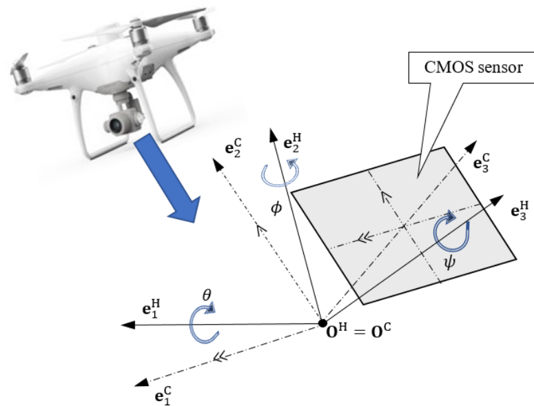
Figure 4. Graphical interpretation of base rotation ( \mathbf{e}_1^C, \mathbf{e}_2^C, \mathbf{e}_3^C ) relative to the base ( \mathbf{e}_1^H, \mathbf{e}_2^H, \mathbf{e}_3^H ) and the method of binding \mathcal{T}^C with the UAV camera projection system.
