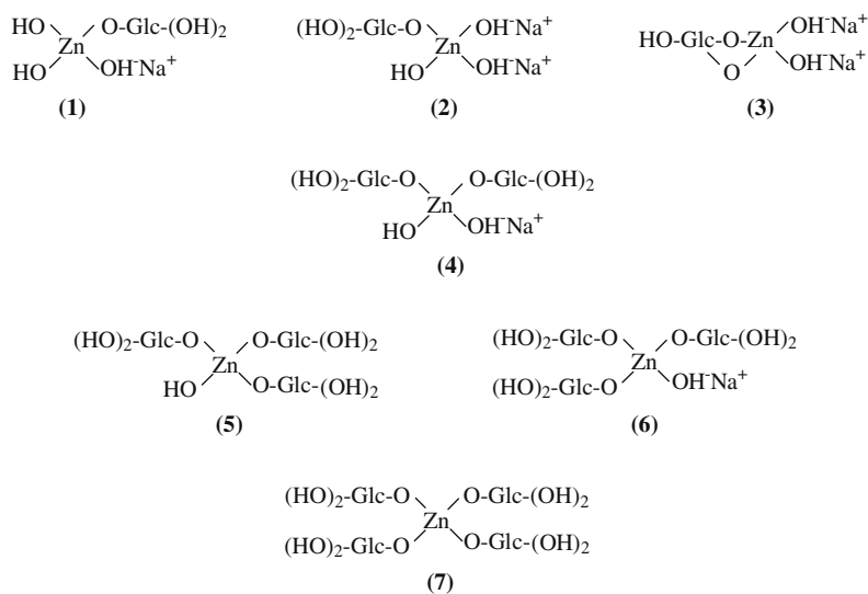
Scheme 1. Possible structures of zincated starch.
