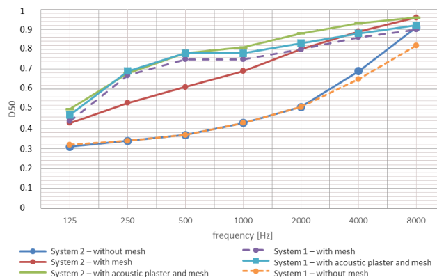
Fig. 18. Average D50 values for the Courtyard with the mesh ; with the mesh plus the acoustic plaster; and without the mesh .
