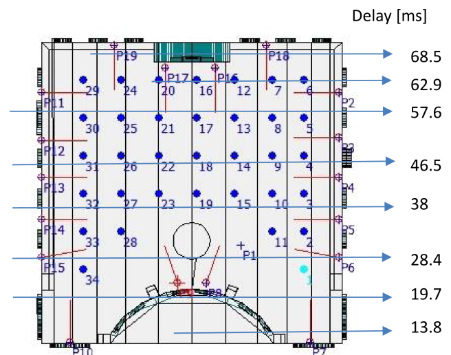
Fig. 10. Distribution of speakers and microphones in the Courtyard.
