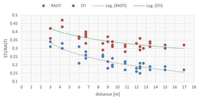
Fig. 3. Dependence of RASTI and STI values on the distance between the source and the measurement point. Speech intelligibility scale: 0–0.3 bad, 0.3–0.45 poor, 0.45–0.6 fair, 0.6–0.75 good, 0.75–1 excellent.
