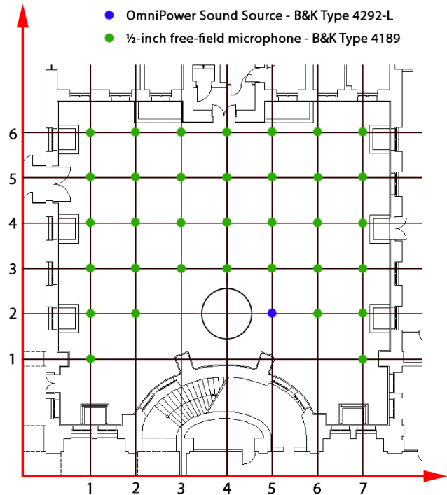
Fig. 1. The grid with measurement points and sound sources. The x - and y -axes reflect axes of STI graphic distributions shown in diagram in Fig. 4.
