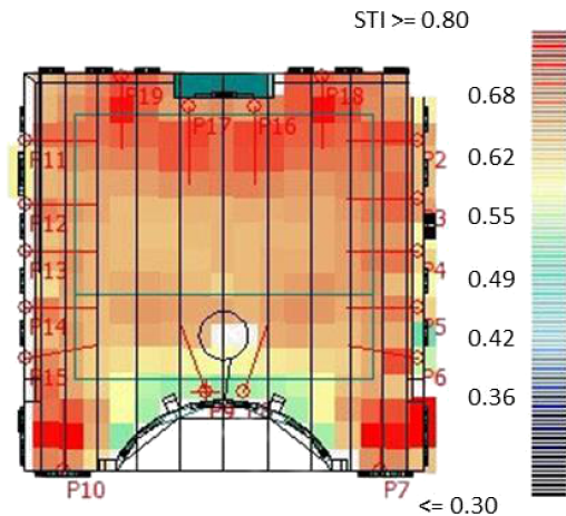
Fig. 22. Graphic distribution of STI in the Courtyard with the suspended metal metal mesh and the acoustic plaster when using system I.
