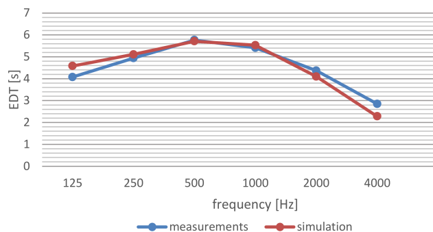
Fig. 8. Comparison of the average EDT value for measurements and simulation.
