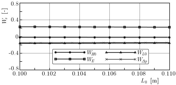
Fig. 10. Relative sensitivity coefficients calculated for M3 model vs. initial cable length L_0
