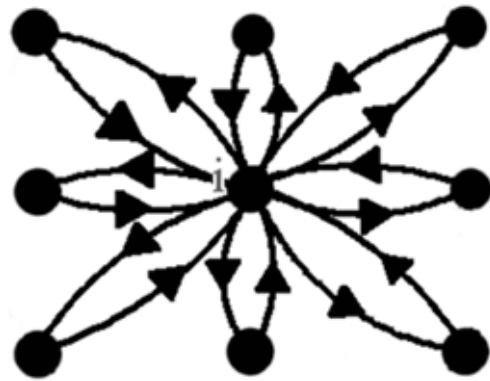
Figure 3. Vertex i and incident outgoing and incoming edges
