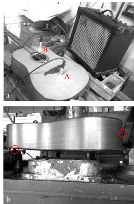
Fig. 5. Guitar support (a) and accelerometer location (b) during excitation in laboratory.
