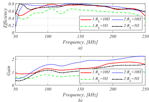
Fig. 10. Experimental results of topologies with the diode (solution 1) and transistor (solution 2): (a) efficiency; (b) voltage gain.
