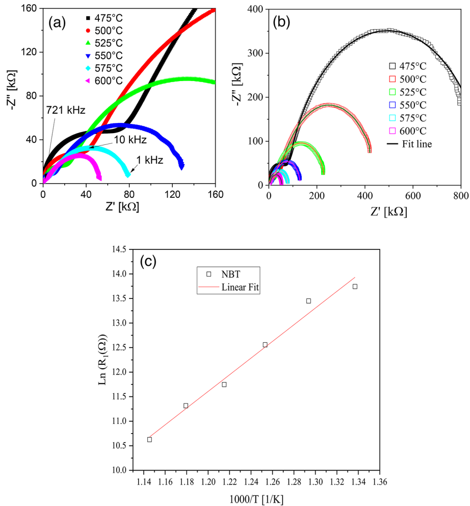
Fig. 10. Nyquist plot of NBT single crystals at selected temperatures, for small Z' , Z' ranges (a) and for full Z' , Z' ranges (b). The solid line represents the data fitted using the equivalent circuit model. The evolution of values R_1 in function of inverse temperature (Arrhenius plot) (c).
