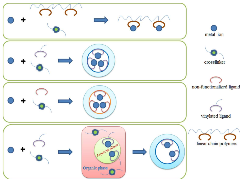
Figure 5. Schematic representation of different approach to IIPs preparation (Branger et al., 2013; Płotka-Wasyłka et al., 2016a).
