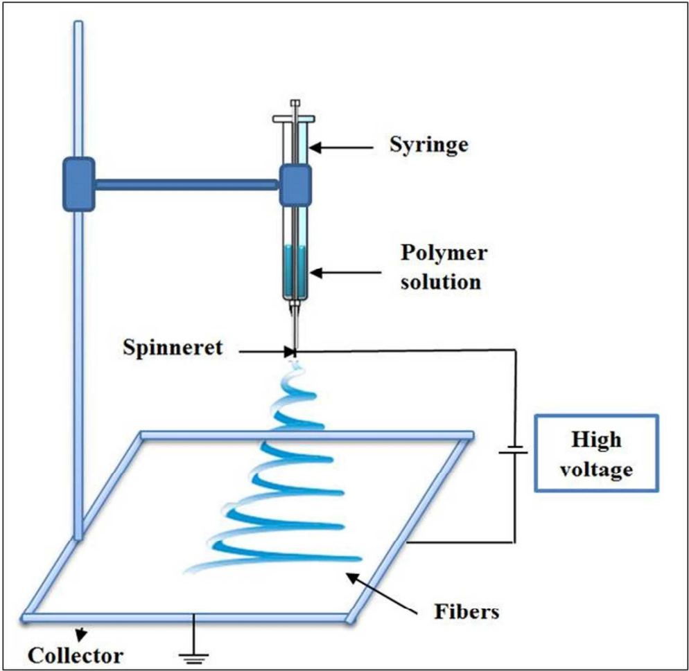
Figure 6. Schematic representation illustrating the set up of an electrospinning apparatus.
