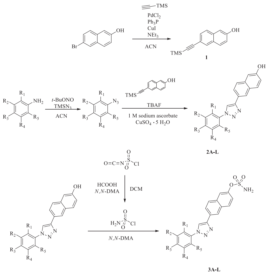
Scheme 1. Synthesis of 6-((trimethylsilyl)ethynyl)naphthalen-2-ol 1 and 6-(1-phenyl-1 H -1,2,3-triazol-4-yl)naphthalen-2-yl sulphamate derivatives (R 1 , R 2 , R 3 , R 4 , R 5 = H, F, Cl, or Br) 3A-L .
