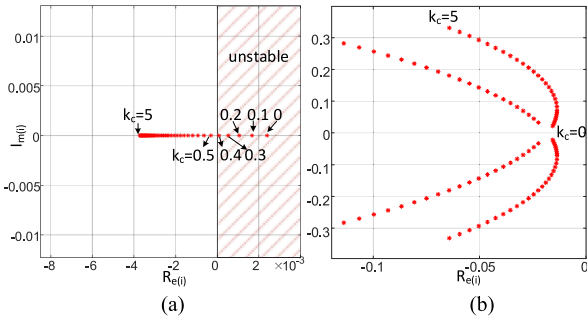
Fig. 7. Spectrum of matrix A of the linearized observer system for \omega_r = 0.03 , T_L = -0.8 , c_\alpha = 1.0 , c_\psi = 0.2 , k_c = 0 \dots 5 p.u.. (a) AFO. (b) NAFO.
