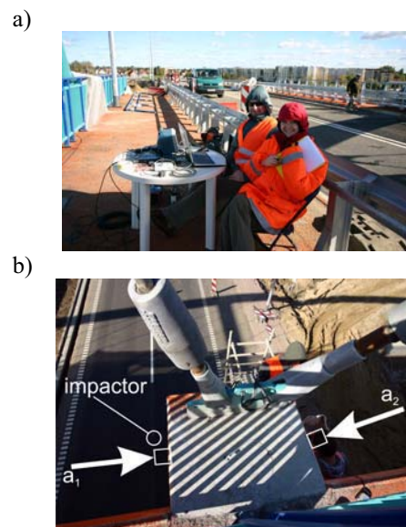
Fig. 4. Field tests: a) instrumentation setup; b) cantilever under examination
