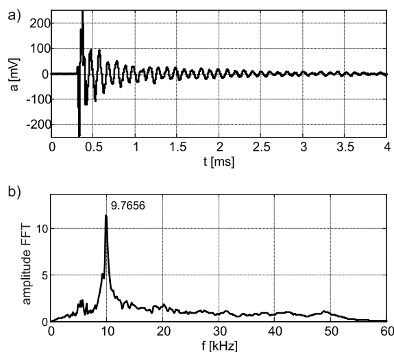
Fig. 9. Acceleration signals measured in point 98: a) in time domain; b) in frequency domain
