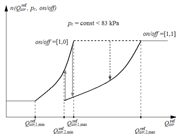
Figure 12. Static characteristics of inverse model of aeration system
