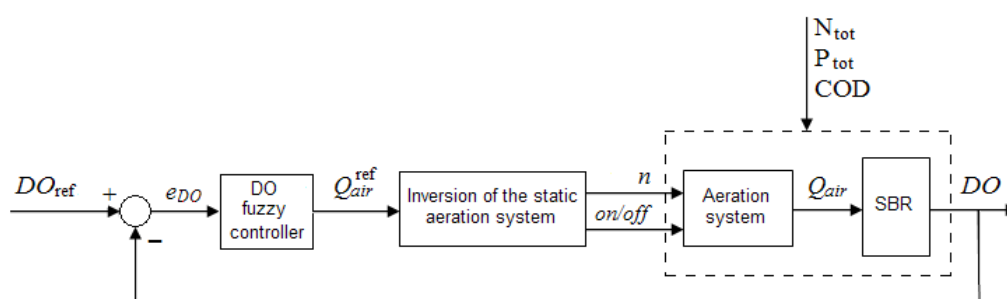
Figure 11. Structure of new control system
