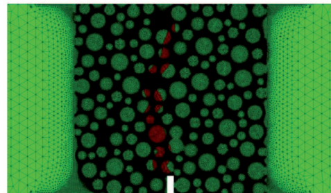
Fig. 20. Effect of aggregate stiffness on force-deflection curve and distribution of non-local strain measure close to beam notch: a) strong circular aggregate, b) weak circular aggregate (fine-grained concrete beam 80 \times 320 \text{ mm}^2 , l_c = 1.5 \text{ mm} , circular aggregate distribution 'c' of Fig. 2 with d_{50} = 4 \text{ mm} and d_{max} = 10 \text{ mm} , \rho = 60\% ).
