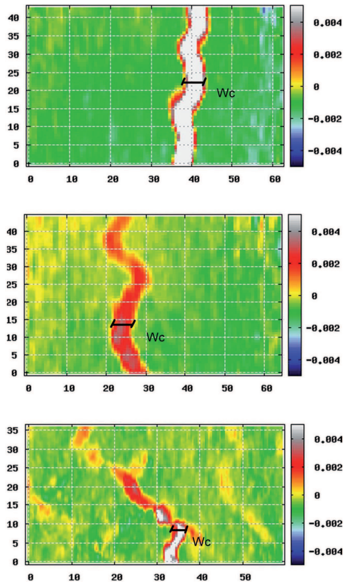
Fig. 4. Formation of localized zone with mean width of w_c \approx 3.5\text{--}4.0 mm directly above notch in 3 different experiments with small-size notched beam 80 \times 320 \times 40 mm 3 using DIC (vertical and horizontal axes denote coordinates in [mm] and colour scales strain intensity) (Skarżyński et al. [14]).
