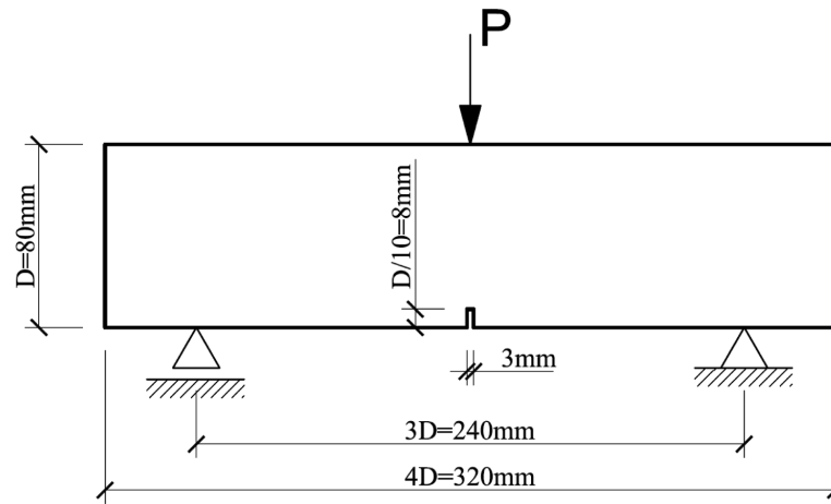
Fig. 1. Geometry of small-size notched concrete beam with thickness of 40 mm subjected to quasi-static three-point bending used in tests by Le Bellėgo et al. [26] and Skarżyński et al. [14] ( P – vertical force, D=80 mm – beam height).
