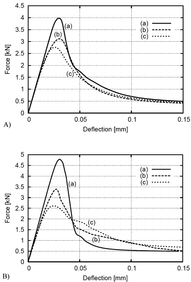
Fig. 18. Numerical effect of notch size on force-deflection curve for two different aggregate densities: a) 0\times 0 mm 2 , b) 3\times 3 mm 2 and c) 6\times 3 mm 2 , A) \rho=30\% , B) \rho=60\% (fine-grained concrete beam 80\times 320 mm 2 , l_c=1.5 mm, circular aggregate distribution 'a' of Fig. 2 with d_{50}=2 mm and d_{max}=8 mm).
