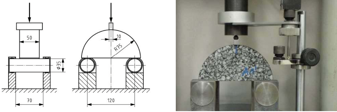
FIGURE 1. Semi-circular specimens
