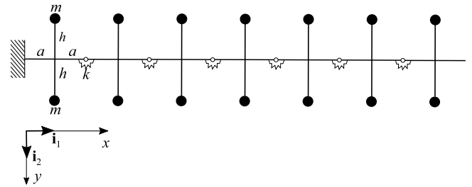
Fig. 4. Cross-beam.
