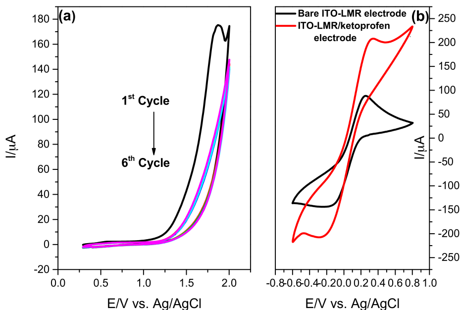
Figure 5. Cyclic voltammograms recorded for (a) ITO-LMR electrode in 0.1 M phosphate buffer saline containing 2 mM of KP for 6 cycles at scan rate of 50 mV·s -1 ; and (b) bare for and KP-modified ITO-LMR in 0.5 M Na 2 SO 4 containing 5 mM [Fe(CN) 6 ] 3-/4- , scan rate 100 mV·s -1 .
