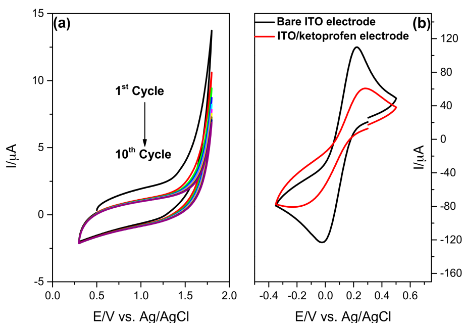
Figure 4. Cyclic voltammograms recorded for (a) ITO electrode in 0.1 M phosphate buffer saline containing 2 mM of KP (10 cycles, scan rate of 50 mV·s -1 ) and (b) ITO and ITO/KP electrode in 0.5 M Na 2 SO 4 containing 5 mM [Fe(CN) 6 ] 3-/4- , scan rate 100 mV·s -1 .
