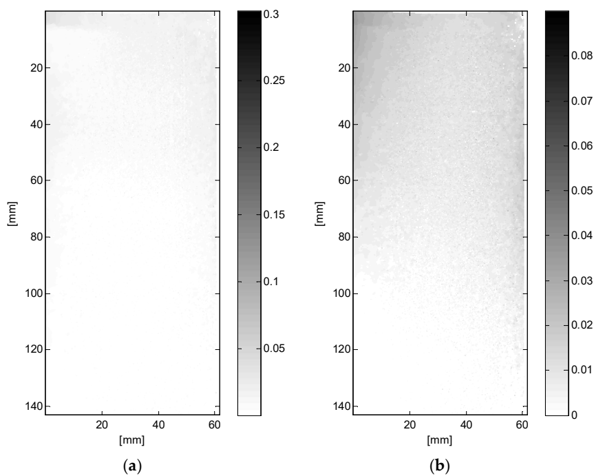
Figure 21. Results of optical flow analysis in full resolution (sample TS1458, grid 801x1861 points). (a) Horizontal displacements [mm] at minimum twist; (b) Corresponding vertical displacements [mm].
