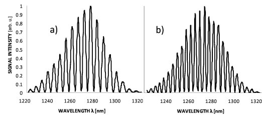
Fig. 3. Measured signal of the blood sample with (a) HCT = 35.2%, (b) HCT = 49.2%.
