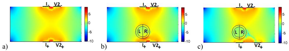
Figure 3. The sensitivity distribution for configuration of the electrode-array given in the figure 2a.
