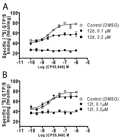
Figure 3. Dose–response curves for CP55,940-induced [ 35 S]GTPγS binding to HEK293 cell membranes expressing the CB1 receptor in the absence and presence of compounds 12d (A) and 12f (B) at the indicated concentrations. Nonspecific binding was determined in the presence of 10 μM unlabeled GTPγS. Data is presented as specific binding of GTPγS (fmol/mg) to the membranes. Each data point represents the mean ± SE (error bars) of at least three independent experiments performed in duplicate.
