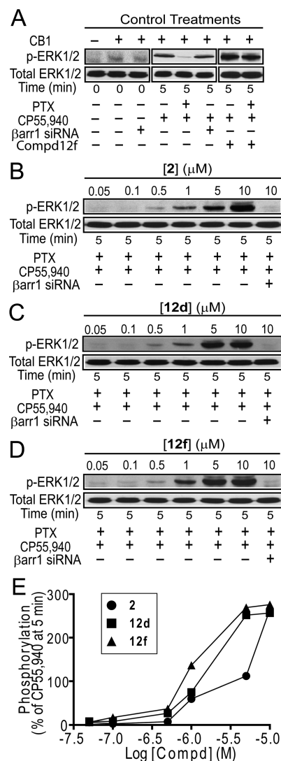
Figure 4. Effect of 12d and 12f on ERK1/2 phosphorylation. (A) Mock-transfected and treatment conditions for CP55,940 (0.2 μM), PTX, and siRNA knockdown of HEK293 cells expressing CB1 are indicated and shown for comparison. (B–D) HEK293 cells expressing CB1 receptors were exposed to 0, 0.05, 0.1, 0.5, 1, 5, and 10 μM of 2 (B), of 12d (C), or of 12f (D) in the presence of 0.2 μM CP55,940 for 5 min with PTX pretreatment for 16 h. Cell lysates were separated on SDS-PAGE and analyzed by Western blots probed with phospho-ERK1/2 (p-ERK1/2). The total level of ERK1/2 was detected for comparison. Note that the two bands correspond to the predominant isoforms, p42 (ERK2) and p44 (ERK1), for ERK1/2. (E) Graphs provide the quantified ERK1/2 phosphorylation levels induced by each compound for 5 min. Data represent the mean ± SE and are expressed as a percent of the level of CP55,940-induced ERK1/2 phosphorylation.
