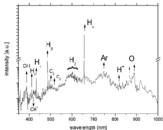
Fig. 4. Typical emission spectra of the \text{H}_2:\text{CH}_4 plasma (microwave power 800 W and gas flow 25 sccm)
