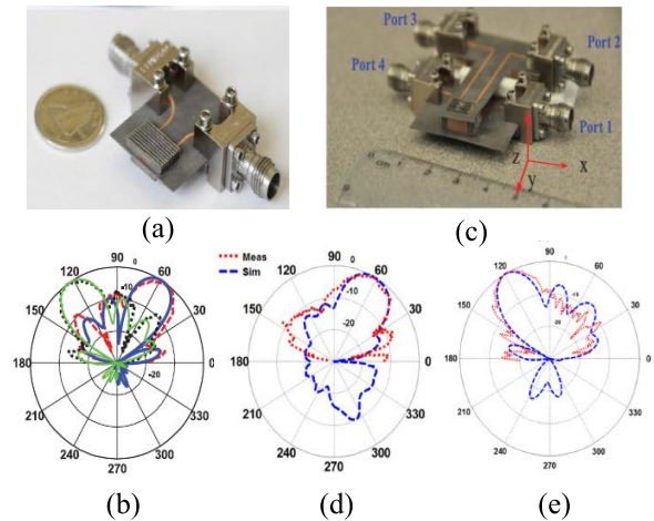
FIGURE 9. The dipole antenna array of [129] with MNZs: (a) the photograph of the double feed dipole antenna with 10 slabs of MNG array: 2 slabs include of 6 \times 4 unit cells and 8 slabs include of 10 \times 4 unit cells, (b) beam steering angles in the E-plane at 60 GHz, (c) the photograph of four feed dipole antenna with eight slabs of MNG where each slab comprise 10 \times 7 unit cells, the simulated and measured deflection angles at 60 GHz (d) in the H-plane, and (e) in the E-plane.
