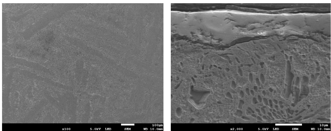
Fig. 11. Cross-sections of Zr-Mn 2 alloy oxidized at 700°C, hydrogen charged and annealed at 400°C
