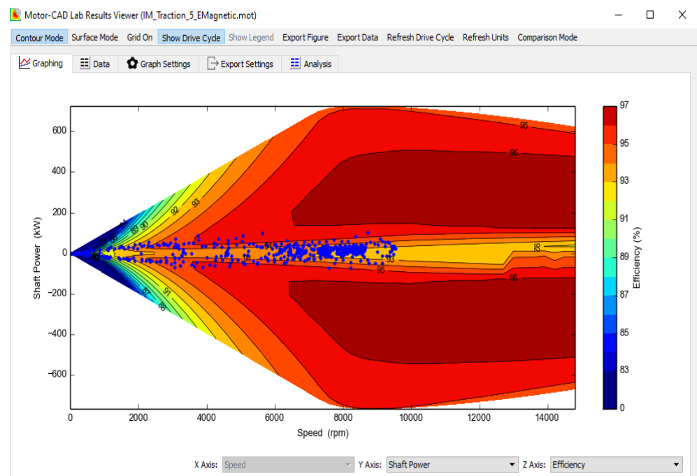
Figure 10. Shaft Power of Designed Motor.
