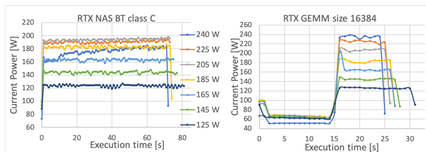
Fig. 1: Sample series of test runs with different Power Limit on RTX system.
