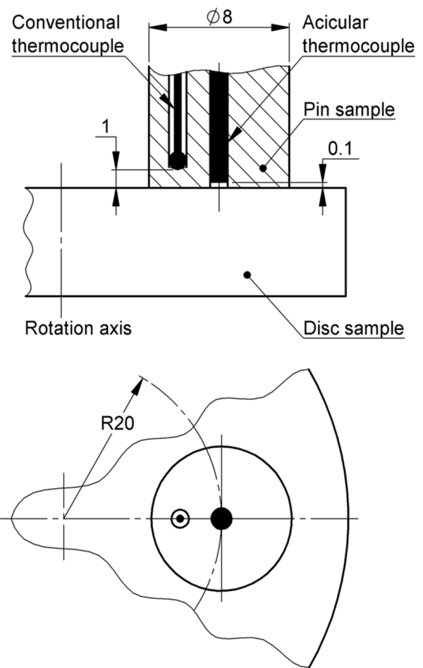
Fig. 3. Initial locations of the acicular and conventional thermocouples in the pin sample.
