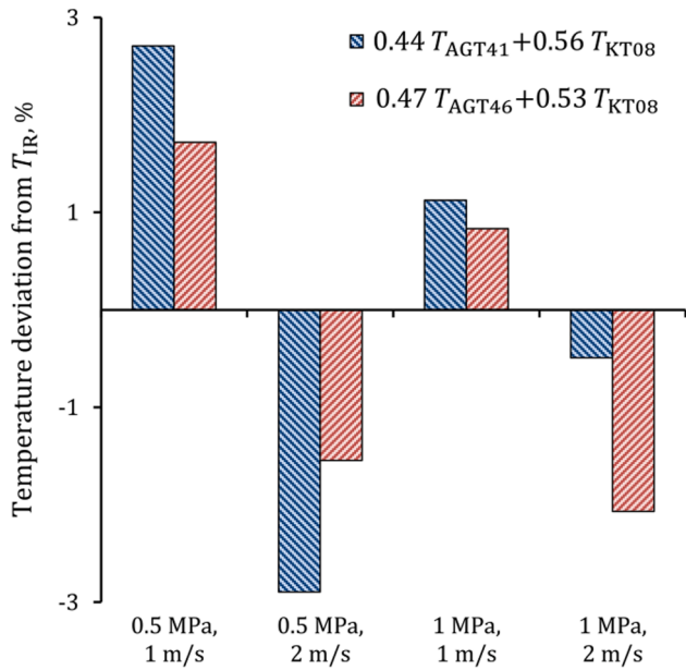
Fig. 14. Deviation of the optimum normalised weighted sum of T_{AGT} and T_{KT08} from T_{IR} .
